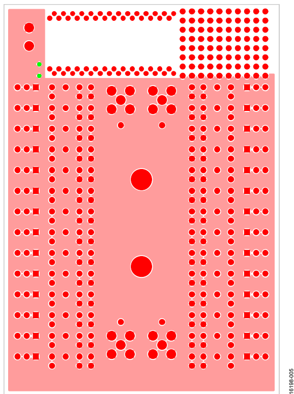
Figure 5. EVAL-28TSSOPEBZ Evaluation Board Bottom Layer
